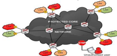
Fig.1. Military Networks
