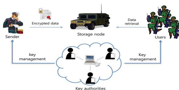
Fig.2: System Architecture.
